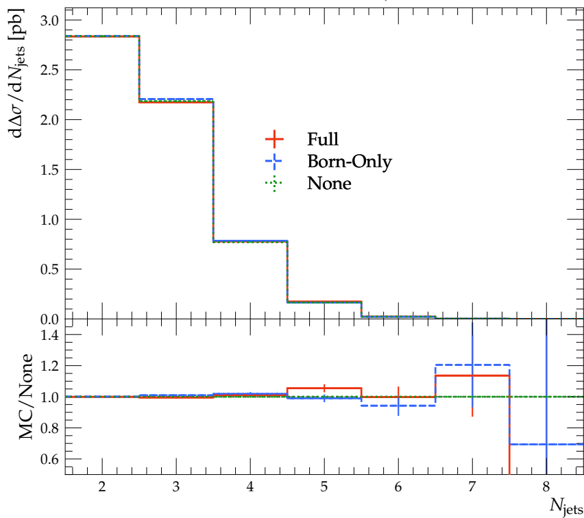
Accepted polarized jet multiplicity d\Delta\sigma/dN_{\text{jets}}
