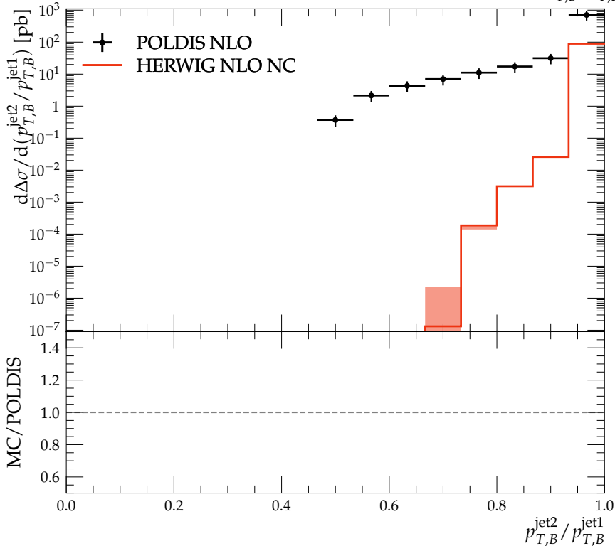
Dijet-selected polarized jet transverse-momentum ratio d\Delta\sigma/d(p_{T,B}^{\text{jet2}}/p_{T,B}^{\text{jet1}})
