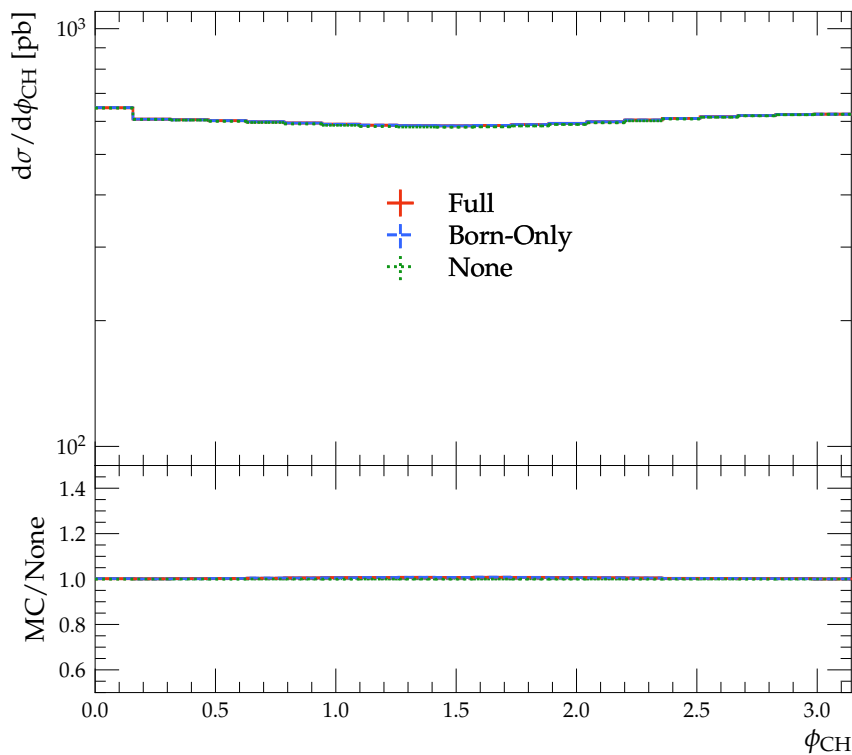
Current-hemisphere particle azimuth relative to the lepton plane d\sigma/d\phi_{CH}
