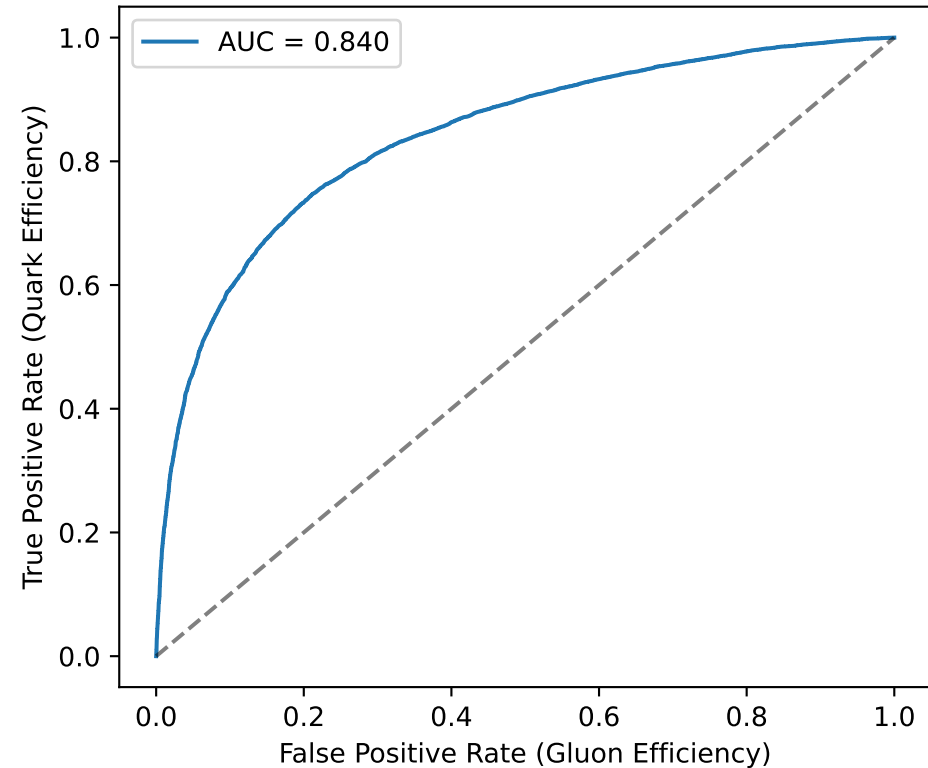
ROC Curve
