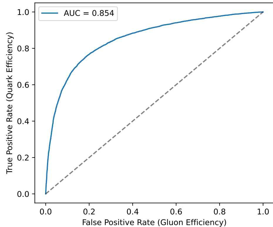
ROC Curve
