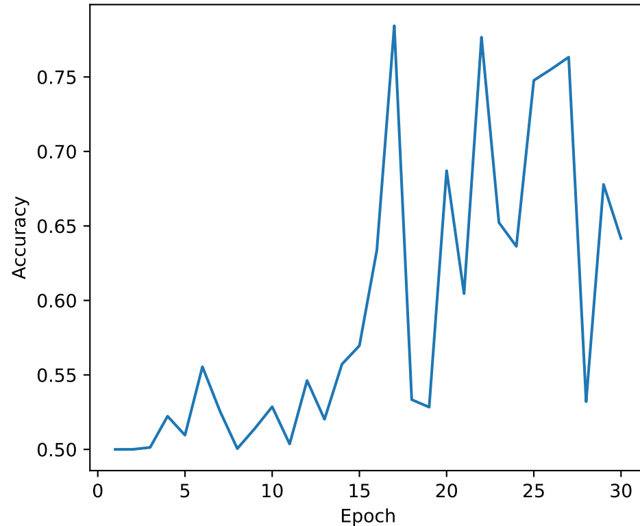
Validation Accuracy
