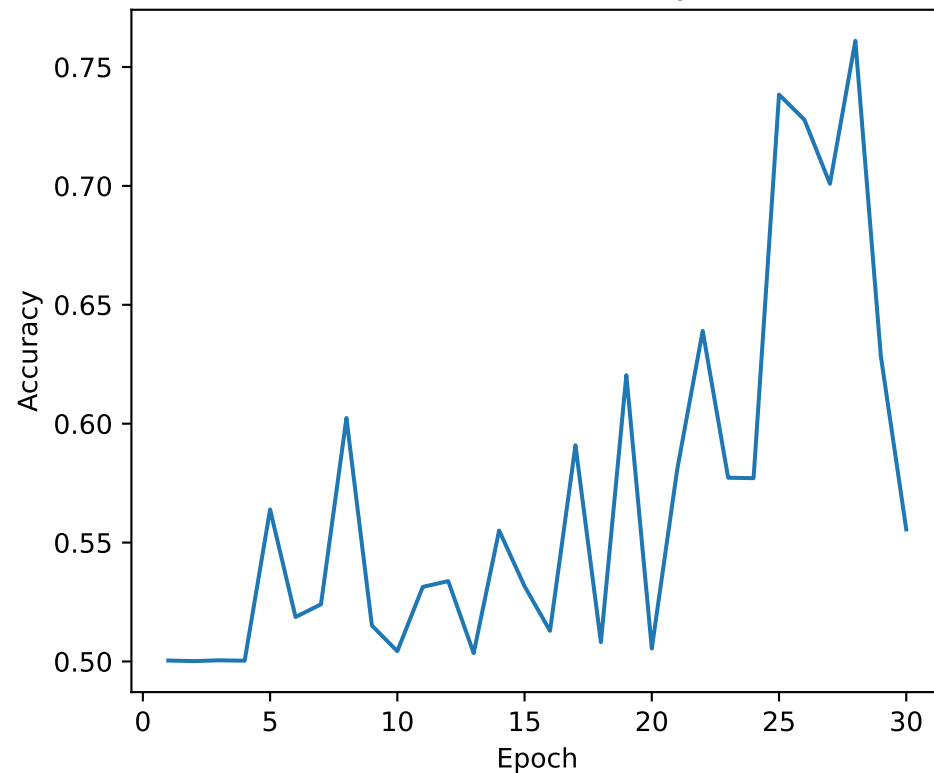
Validation Accuracy
