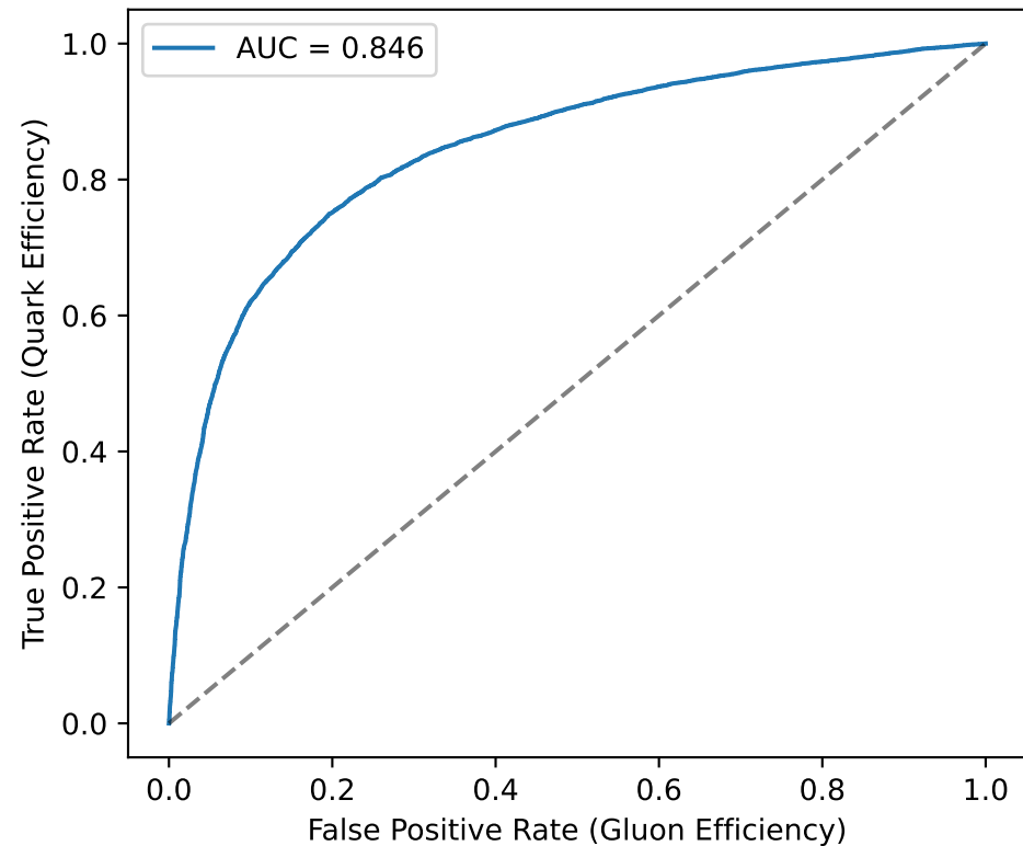
ROC Curve
