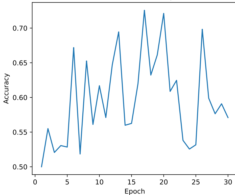
Validation Accuracy
