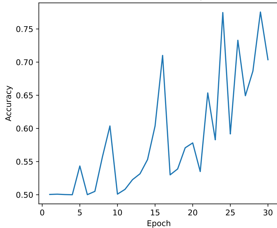
Validation Accuracy
