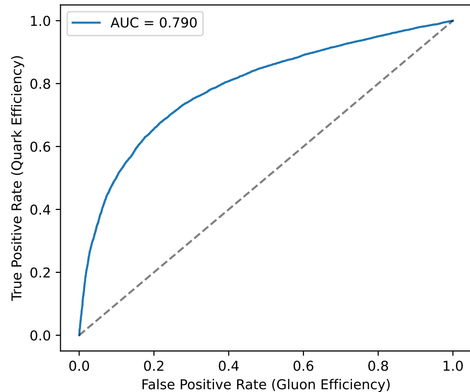
ROC Curve
