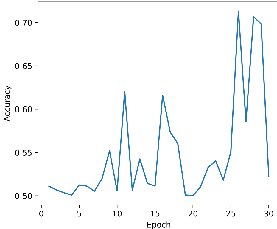
Validation Accuracy
