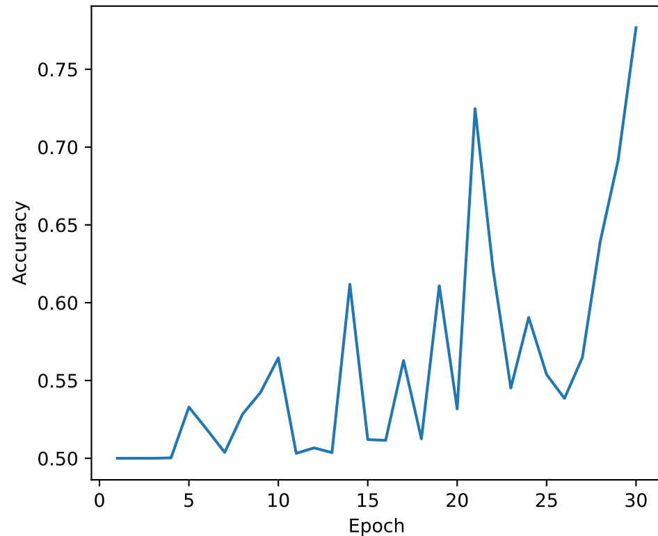
Validation Accuracy
