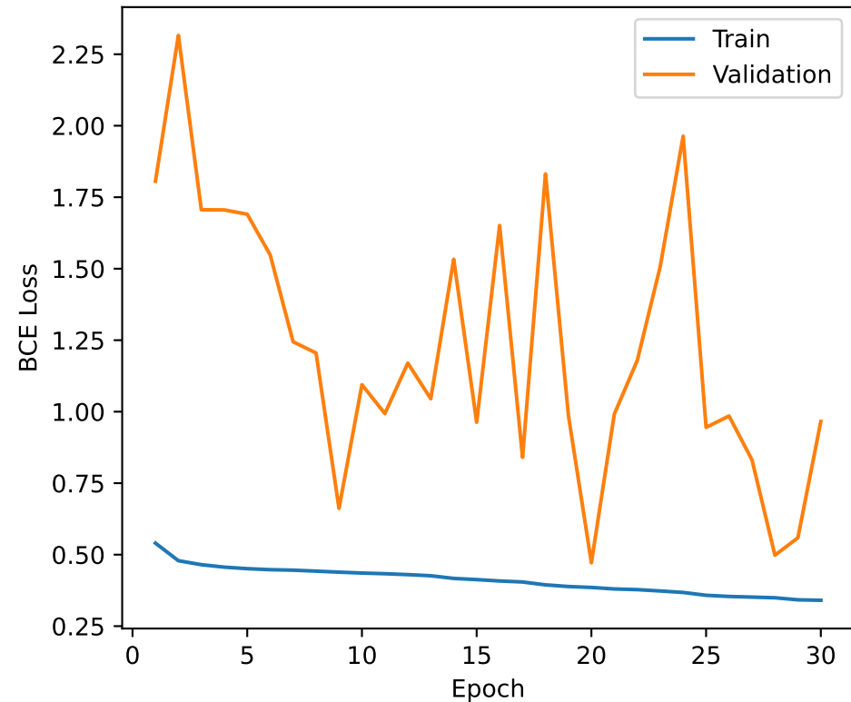
Training and Validation Loss
