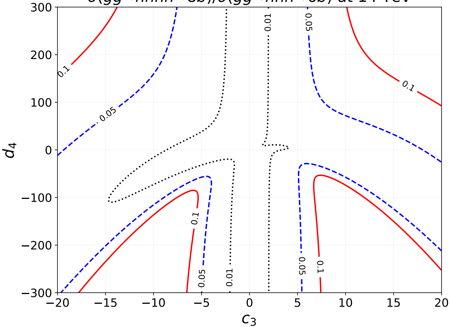
\sigma(gg \rightarrow hhhh \rightarrow 8b) / \sigma(gg \rightarrow hhhh \rightarrow 6b) at 14 TeV
