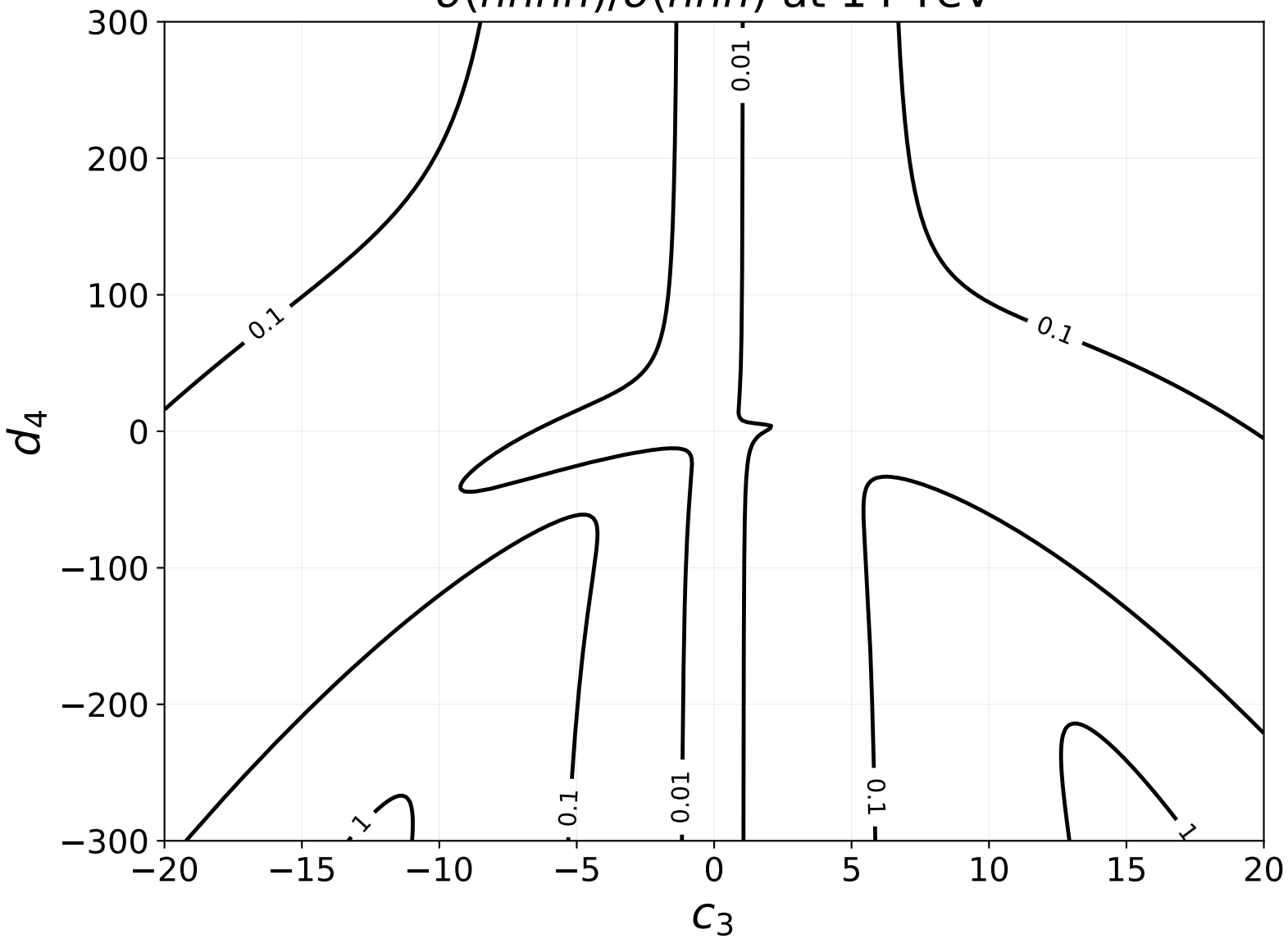
\sigma(hhhh)/\sigma(hhh) at 14 TeV
