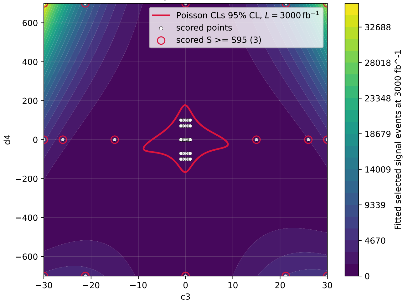
Fitted selected signal events at 3000 fb -1
