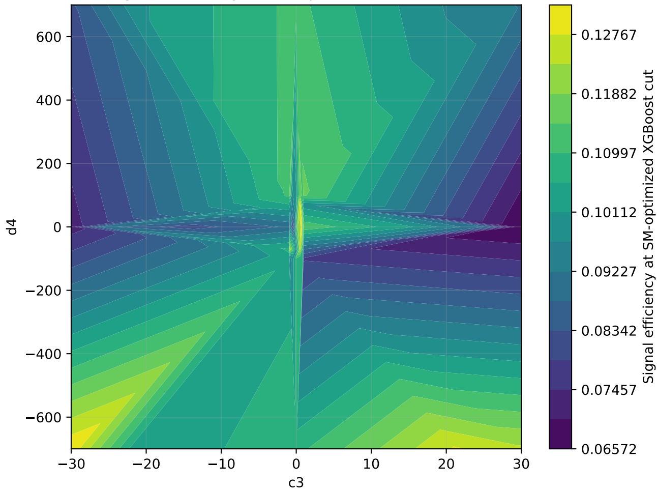
Signal efficiency at SM-optimized XGBoost cut
