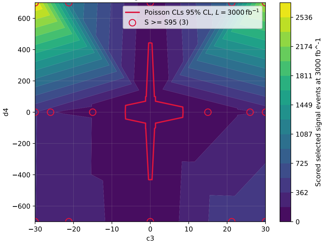
Scored selected signal events at 3000 fb -1
