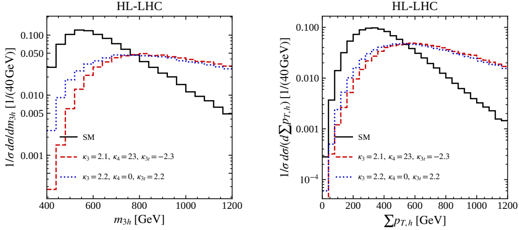
Figure 9: Normalised m_{3h} and \sum p_{T,h} distributions at the HL-LHC for the SM and the two \mu_{3h} \simeq 65 benchmarks (\kappa_3, \kappa_4, \kappa_{3t}) = (2.1, 23, -2.3) and (2.2, 0, 2.2) . The distributions use the same 40 GeV binning and displayed ranges as Figures 7 and 8. We fix \kappa_t = 1 and \kappa_{2t} = 0 .
