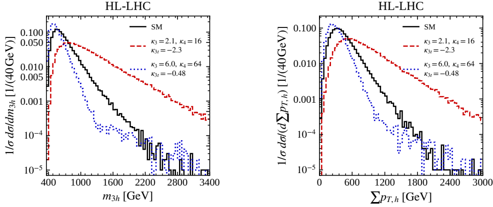
Figure 9: Normalised m_{3h} and \sum p_{T,h} distributions at the HL-LHC for the SM and the two \mu_{3h} \simeq 75 benchmarks (\kappa_3, \kappa_4, \kappa_{3t}) = (2.1, 16, -2.3) and (6.0, 64, -0.48) . The distributions use the same 40 GeV binning as Figures 7 and 8, with wider displayed ranges to retain the hard benchmark's high-energy tail. We fix \kappa_t = 1 and \kappa_{2t} = 0 .
