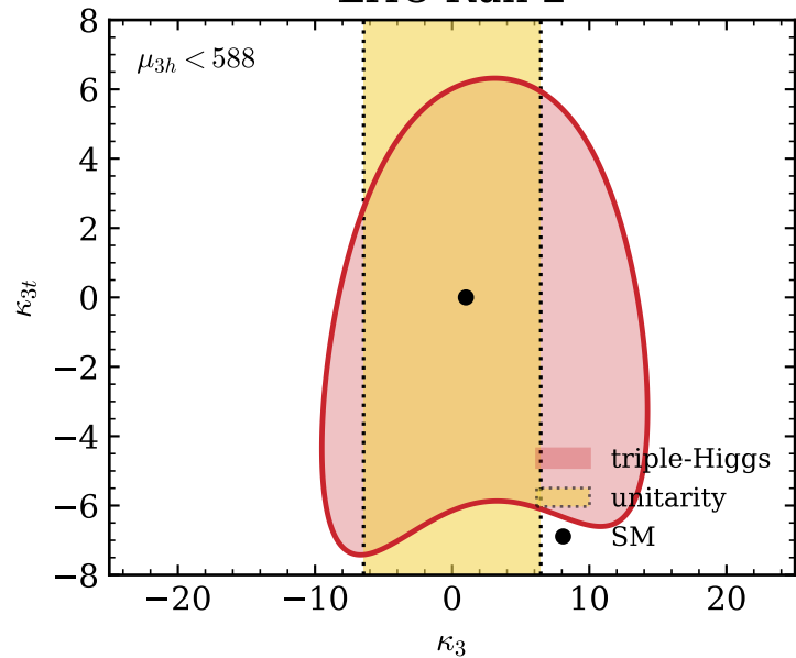
LHC Run 2
