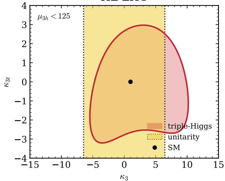
HL-LHC
