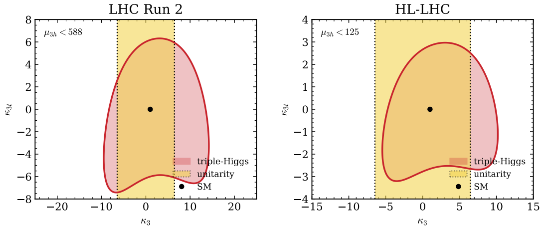
Figure 5: Constraints in the \kappa_3 - \kappa_{3t} plane at LHC Run 2 (left) and the HL-LHC (right), obtained from Eq. (39) using \mu_{3h} < 588 and \mu_{3h} < 125 , respectively. The red regions are allowed by the inclusive triple-Higgs rate, the black points denote the SM, and the yellow vertical bands show the projection of the tree-level hh \rightarrow hh perturbative-unitarity constraint. We fix \kappa_4 = \kappa_t = 1 and \kappa_{2t} = 0 . The yellow band constrains \kappa_3 only; no independent unitarity condition on \kappa_{3t} is imposed.
