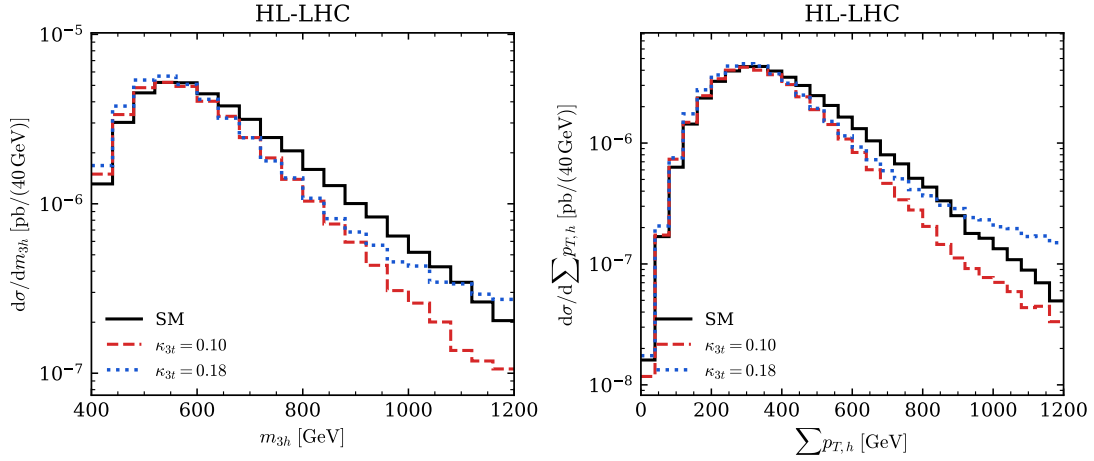
Figure 10: As in Figure 9, but for the unnormalised differential cross sections in pb per 40 GeV bin.
