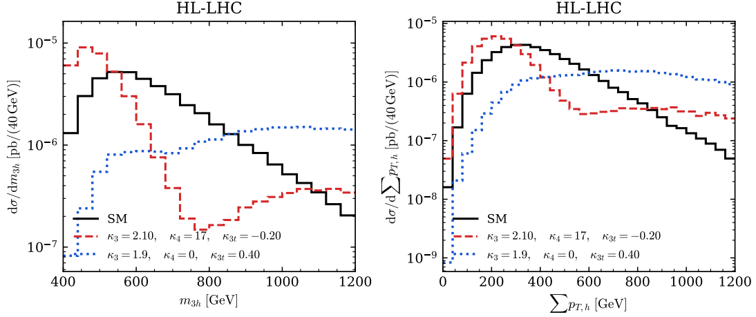
Figure 12: As in Figure 11, but for the unnormalised differential cross sections in pb per 40 GeV bin.
