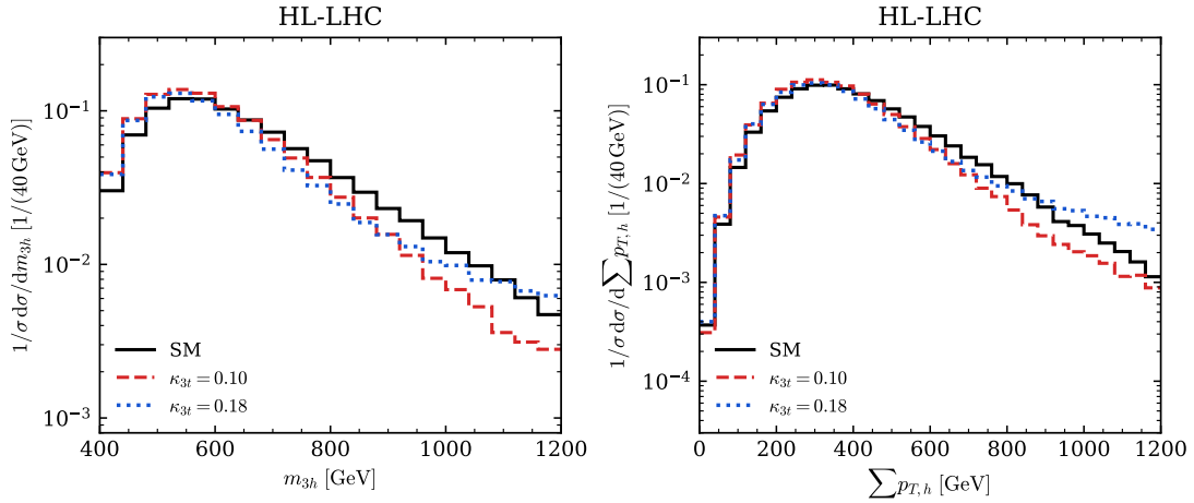
Figure 9: Normalised m_{3h} and \sum p_{T,h} distributions at the HL-LHC for the SM and for \kappa_{3t} = 0.10 and 0.18 . We fix \kappa_3 = \kappa_4 = \kappa_t = 1 and \kappa_{2t} = 0 . Each curve contains 100 000 generated events and uses 40 GeV bins.
