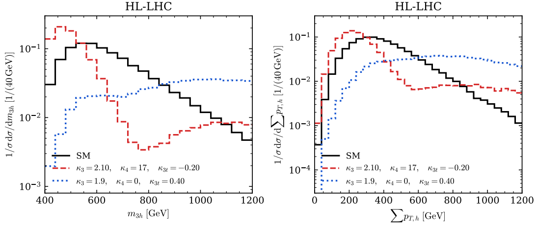
Figure 11: Normalised m_{3h} and \sum p_{T,h} distributions at the HL-LHC for the SM and the two rate-matched benchmarks (\kappa_3, \kappa_4, \kappa_{3t}) = (2.10, 17, -0.20) and (1.9, 0, 0.40) . We fix \kappa_t = 1 and \kappa_{2t} = 0 . Each curve contains 100 000 generated events.
