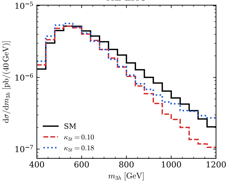
HL-LHC
