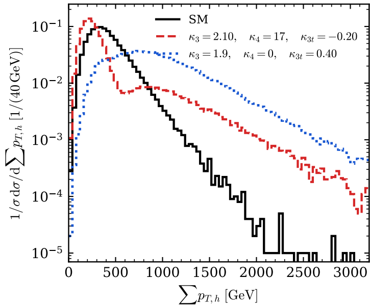
HL-LHC
