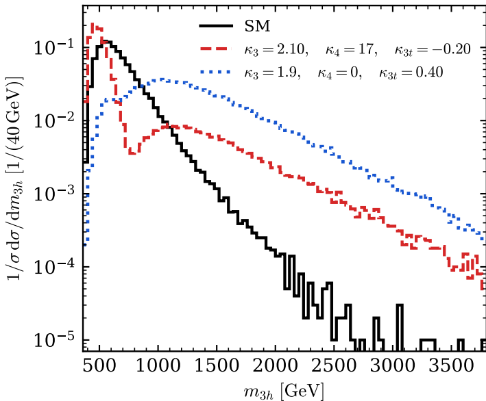
HL-LHC
