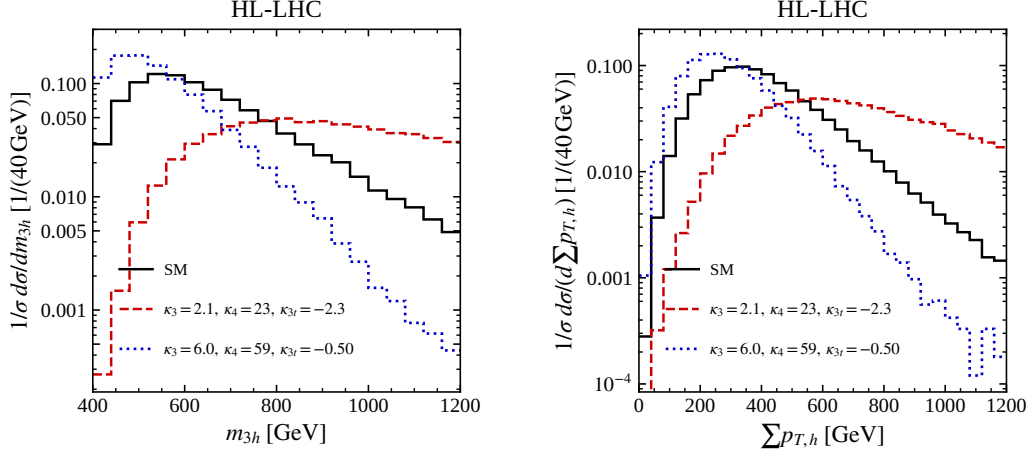
Figure 9: Normalised m_{3h} and \Sigma p_{T,h} distributions at the HL-LHC for the SM and the two \mu_{3h} \simeq 65 benchmarks (\kappa_3, \kappa_4, \kappa_{3t}) = (2.1, 23, -2.3) and (6.0, 59, -0.50) . The distributions use the same 40 GeV binning and plotting ranges as Figures 7 and 8. We fix \kappa_t = 1 and \kappa_{2t} = 0 .
