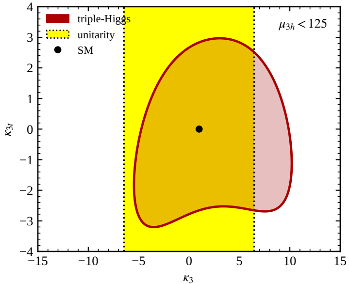
HL-LHC
