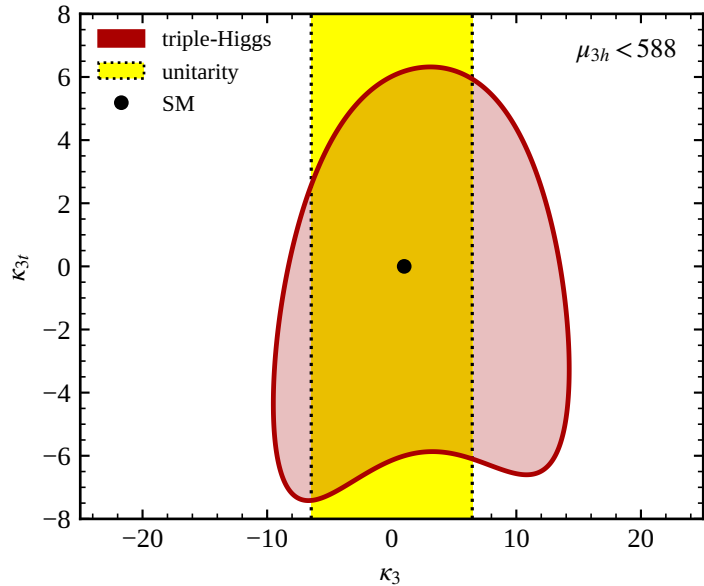
LHC Run 2
