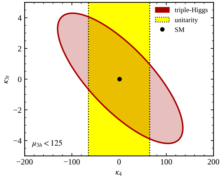
HL-LHC
