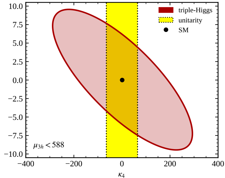
LHC Run 2
