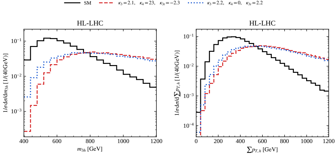
Figure 9: Normalised m_{3h} and \sum p_{T,h} distributions at the HL-LHC for the SM and the two \mu_{3h} \simeq 65 benchmarks (\kappa_3, \kappa_4, \kappa_{3t}) = (2.1, 23, -2.3) and (2.2, 0, 2.2) . The distributions use the same 40 GeV binning and displayed ranges as Figures 7 and 8. We fix \kappa_t = 1 and \kappa_{2t} = 0 .
