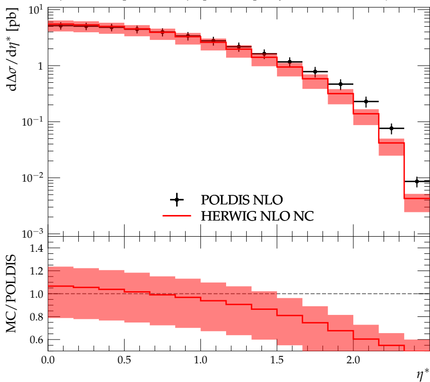
Dijet-selected polarized dijet pseudorapidity difference d\Delta\sigma/d\eta^*
