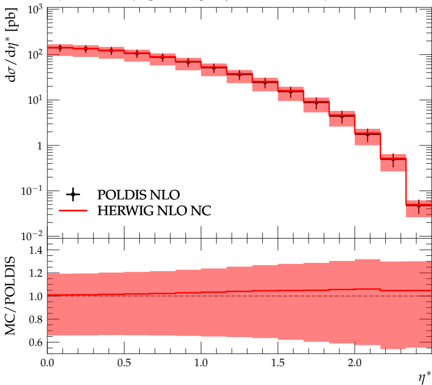
Dijet-selected dijet pseudorapidity difference d\sigma/d\eta^*
