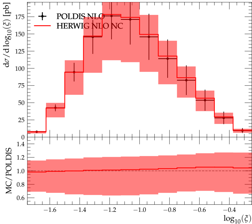
Dijet-selected dijet momentum fraction d\sigma/d\log_{10}(\xi)
