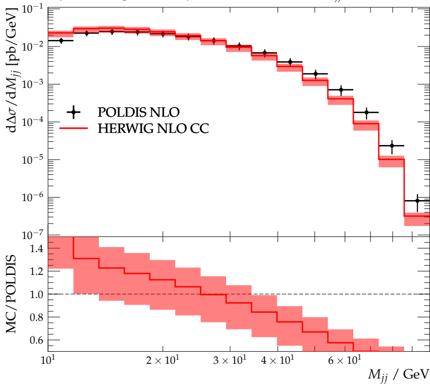
Dijet-selected polarized dijet invariant mass d\Delta\sigma/dM_{jj}
