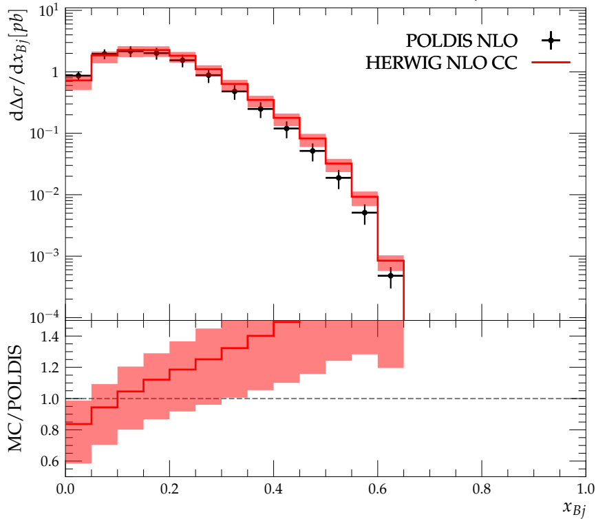
Dijet-selected polarized Bjorken- x distribution d\Delta\sigma/dx_{Bj}
