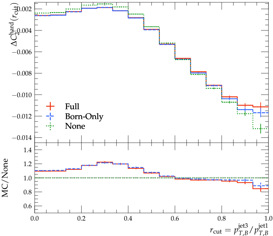
Spin-dependent hard-plane C_2 tail moment
