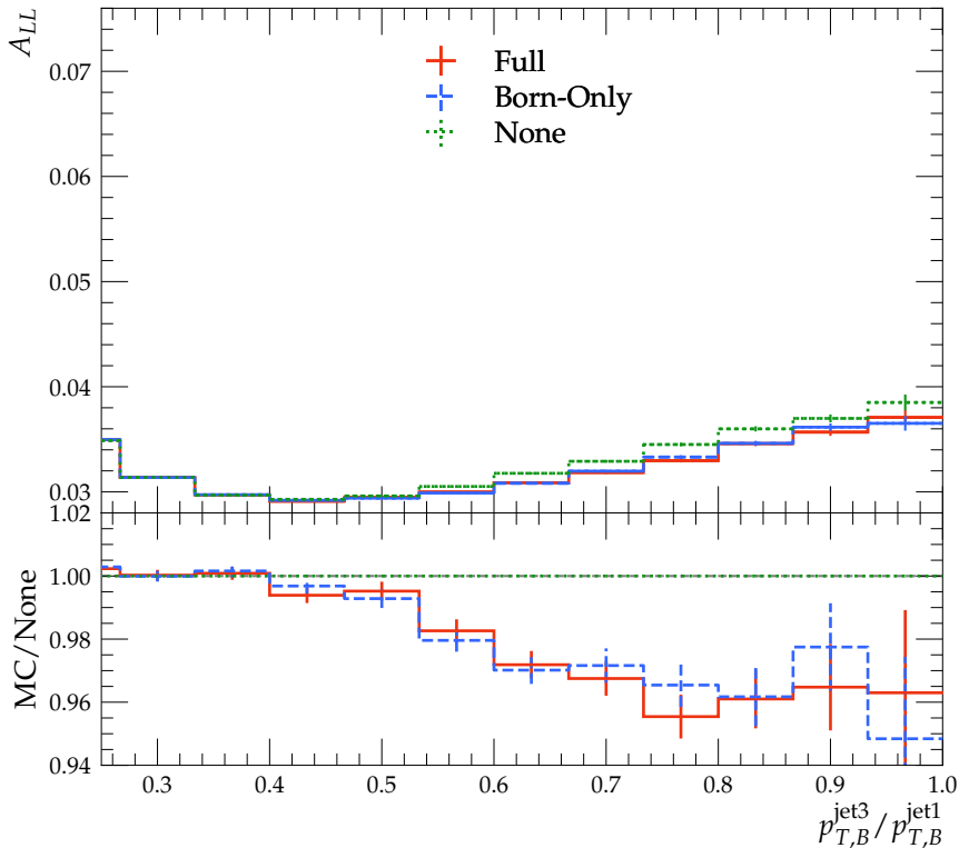
Double-spin asymmetry A_{LL}(p_{T,B}^{\text{jet3}}/p_{T,B}^{\text{jet1}})
