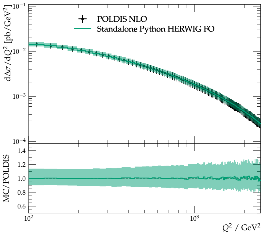
Dijet-selected polarized DIS cross section d\Delta\sigma/dQ^2
