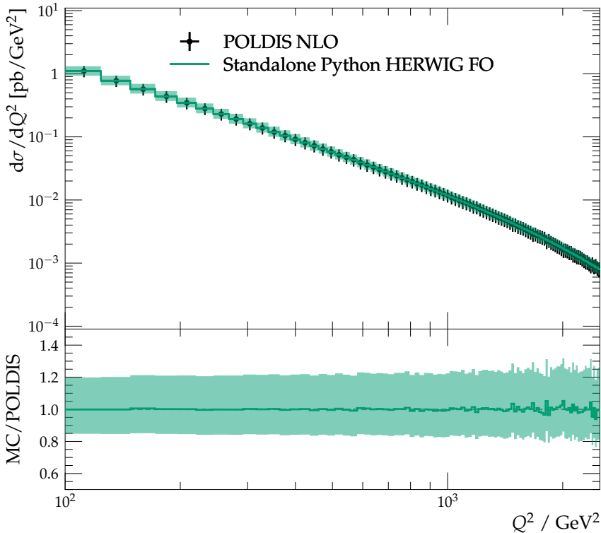
Dijet-selected DIS cross section d\sigma/dQ^2
