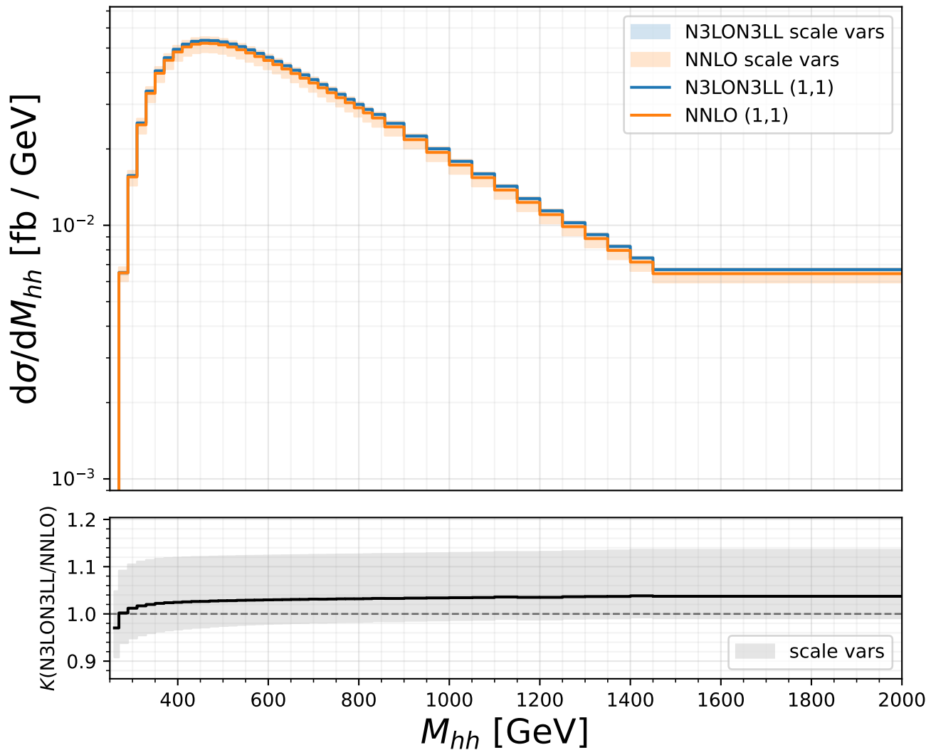
M_{hh} distribution, \sqrt{s} = 13.6 TeV, PDF4LHC21_40, m_H = 125 GeV
