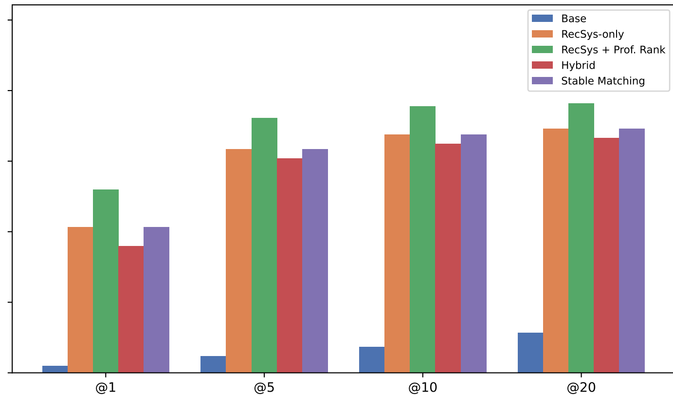
NDCG@K
