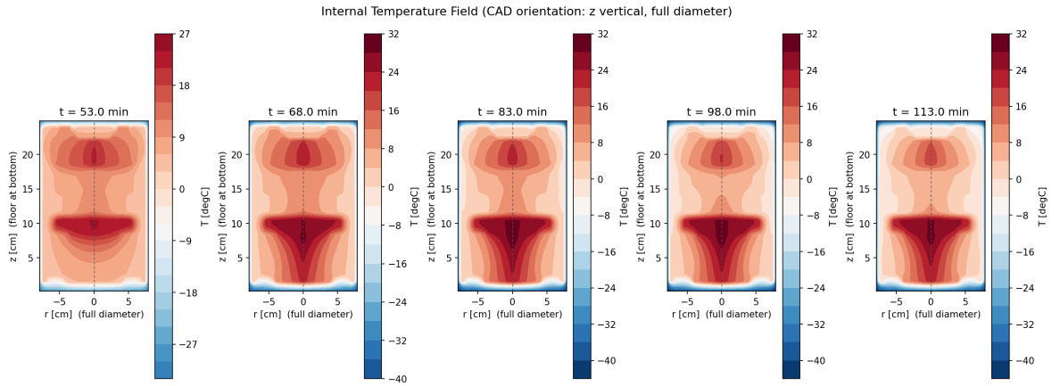
Figure 4: Internal temperature field (CAD orientation, full diameter) at five mission times. With the OBC unpowered during ascent the cavity tracks the cooling wall; the warm bottom-row core appears only after the OBC is energised at 16 km.
