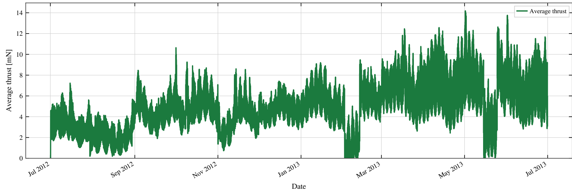
GOCE Staged Mission Profile — Continuous Variable Thrust
