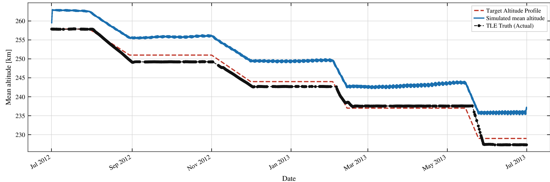
GOCE Staged Mission Profile — Mean Altitude Tracking
