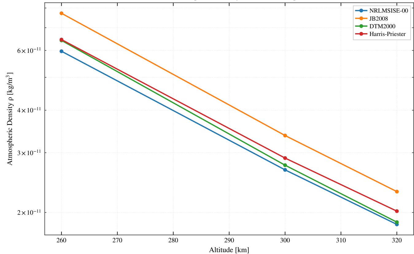
EMV-01: Atmospheric Density vs Altitude Comparison
