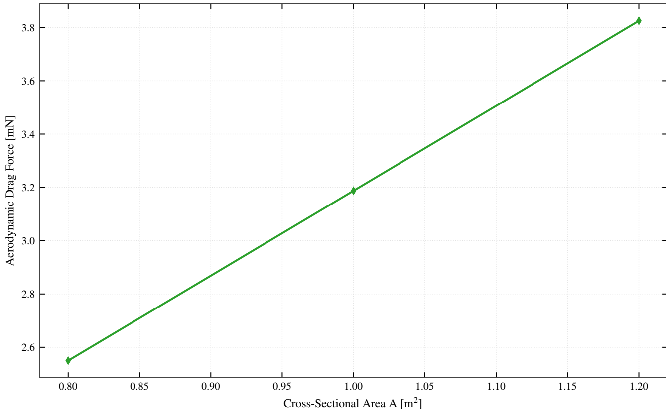
EMV-05: Drag Sensitivity to Cross-Sectional Area at 300 km
