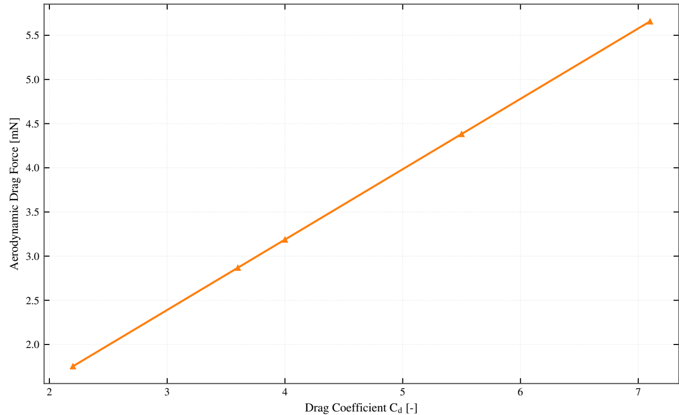
EMV-04: Drag Sensitivity to C_d at 300 km
