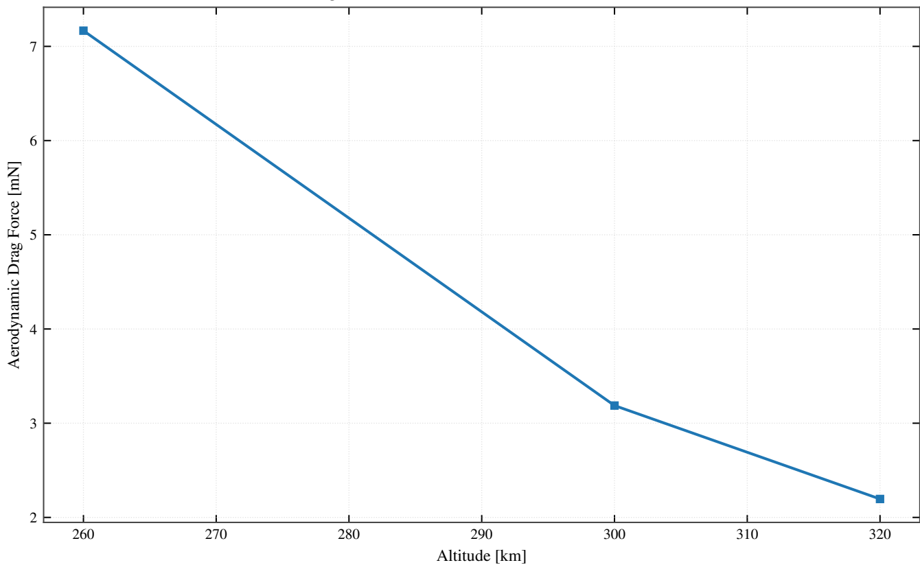
EMV-03: Drag Force vs Altitude (NRLMSISE-00, C_d=4.0 , A=1.0 \text{ m}^2 )
