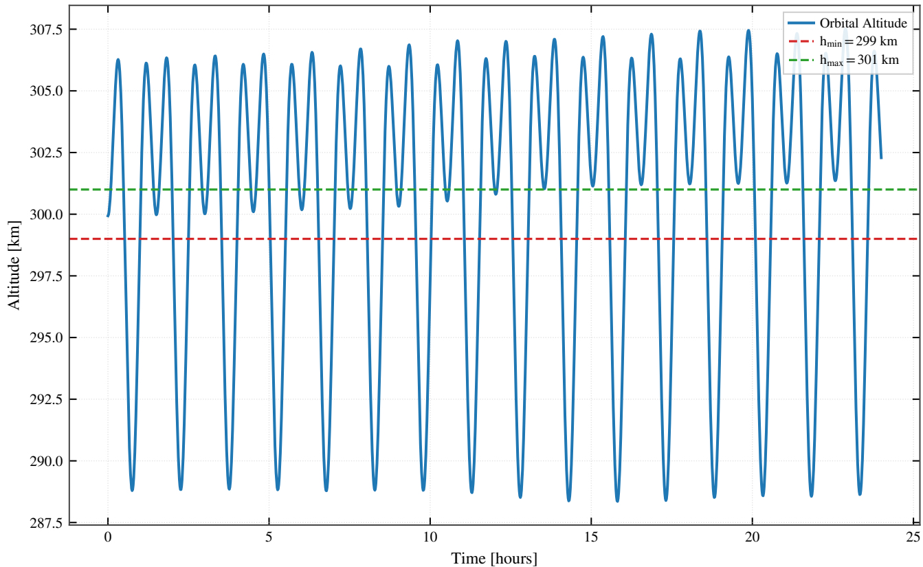
IMV-08: Altitude Control &amp; Threshold Band in VLEO
