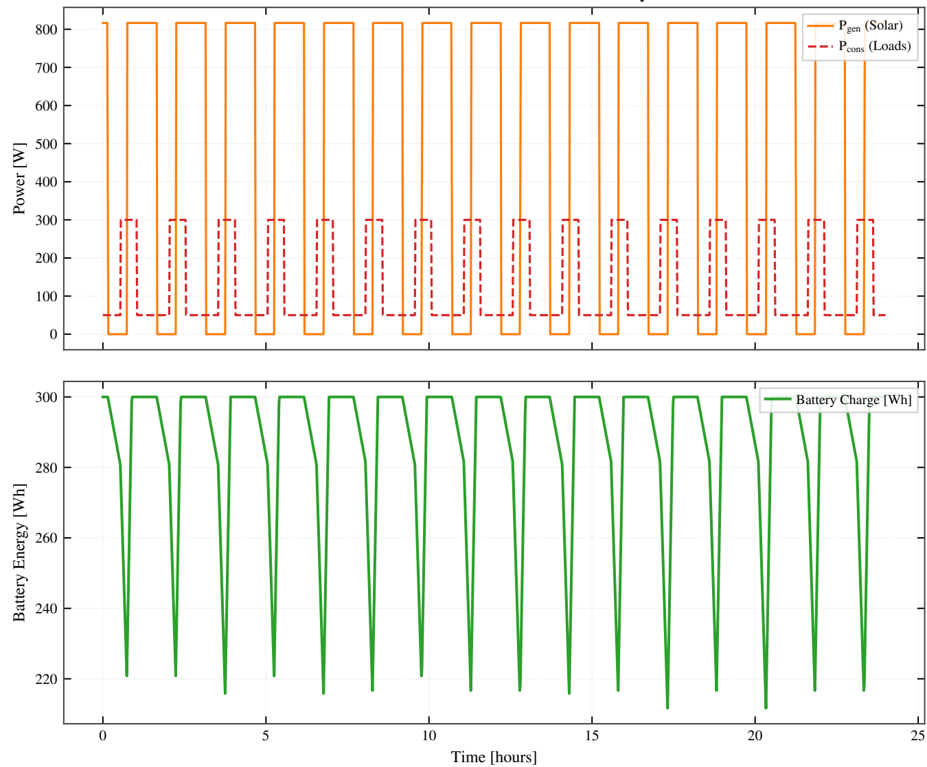
IMV-08: Electrical Power Generation and Battery State
