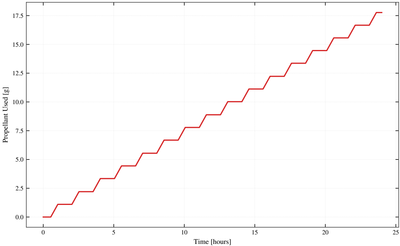
IMV-08: Propellant Mass Consumption Over Mission
