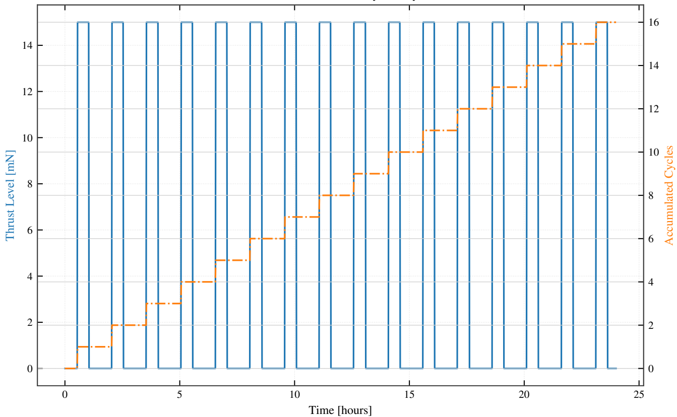
IMV-08: Thruster Activity and Cycles
