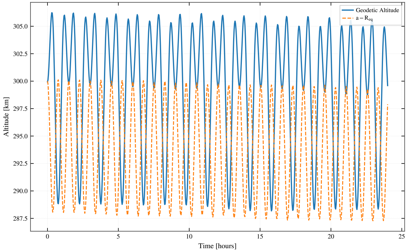
OAV-01: Orbital Altitude Evolution in VLEO (300 km)
