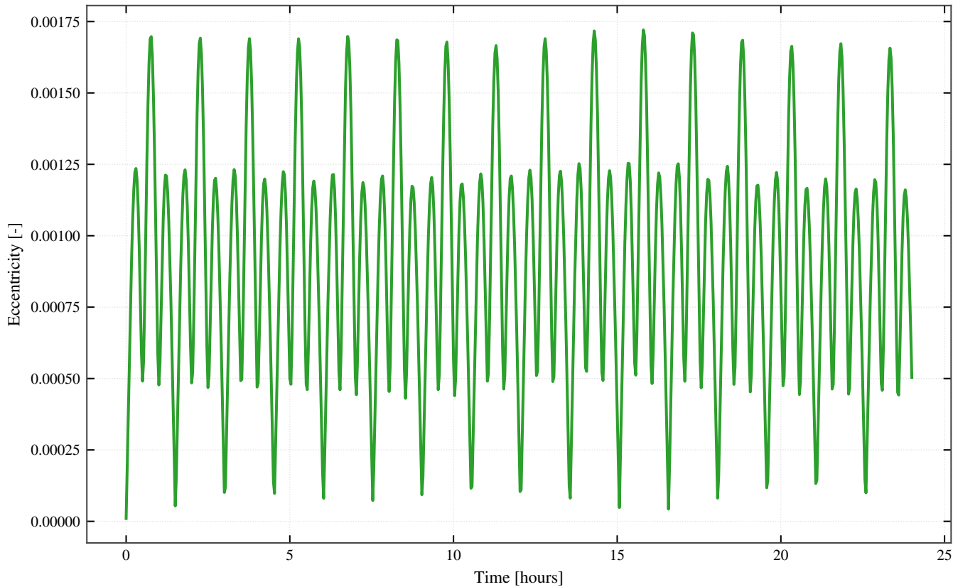
OAV-02: Orbital Eccentricity Evolution
