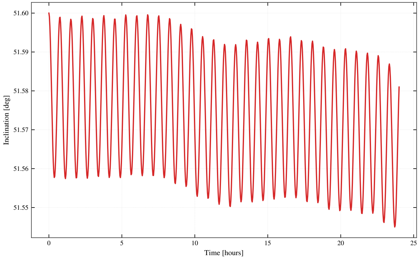
OAV-03: Orbital Inclination Evolution
