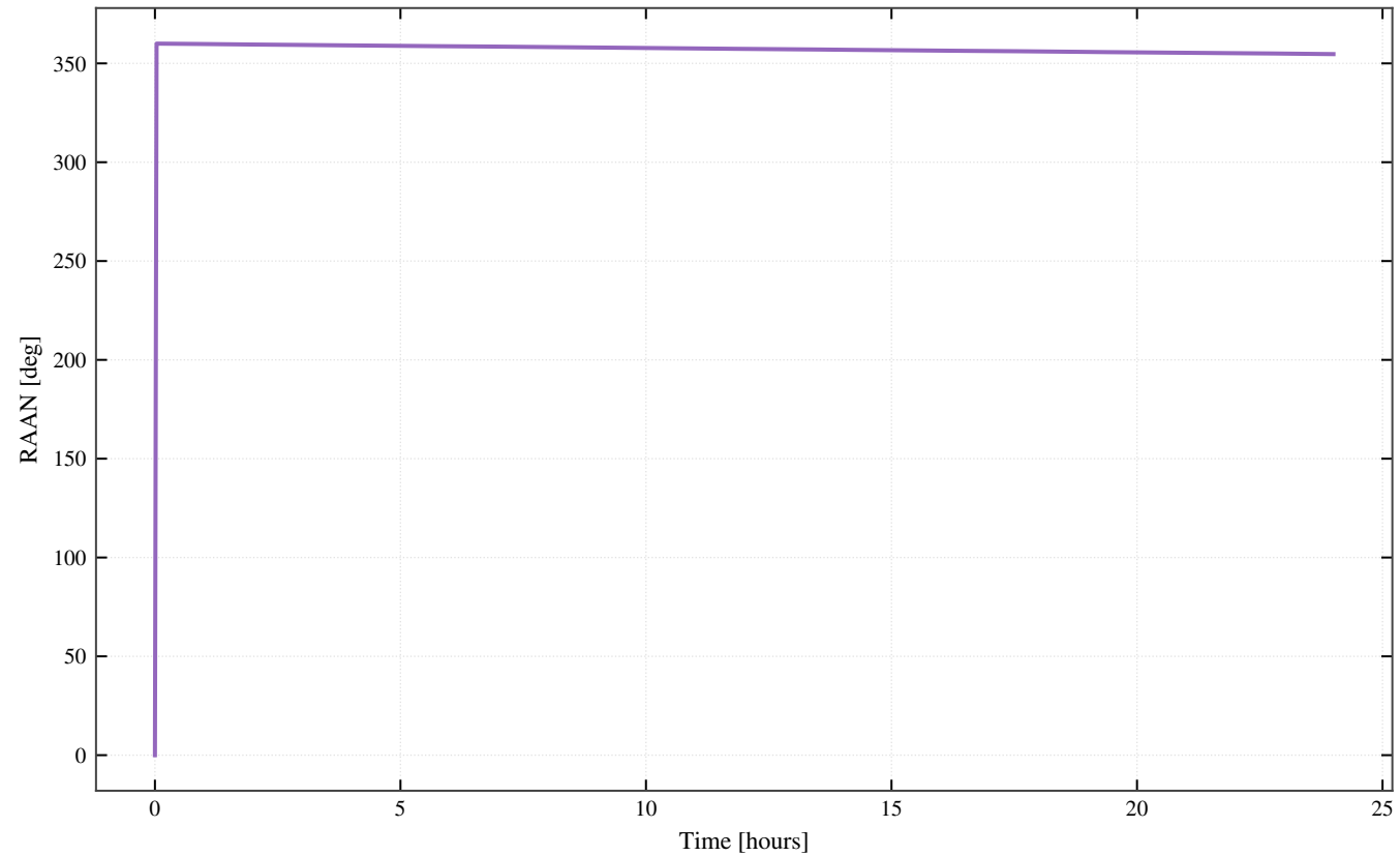
OAV-06: RAAN Secular Drift
