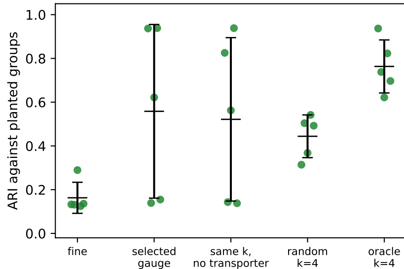
(b) Recovery and controls
