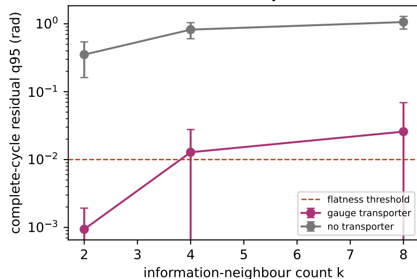
(c) Global consistency across scale
