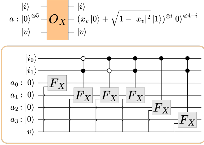
FIG. 1. Oracle O_X action in detail. The implementation of O_X requires the usage of a work register with d' -qubits, that has been omitted here, but explained below.
