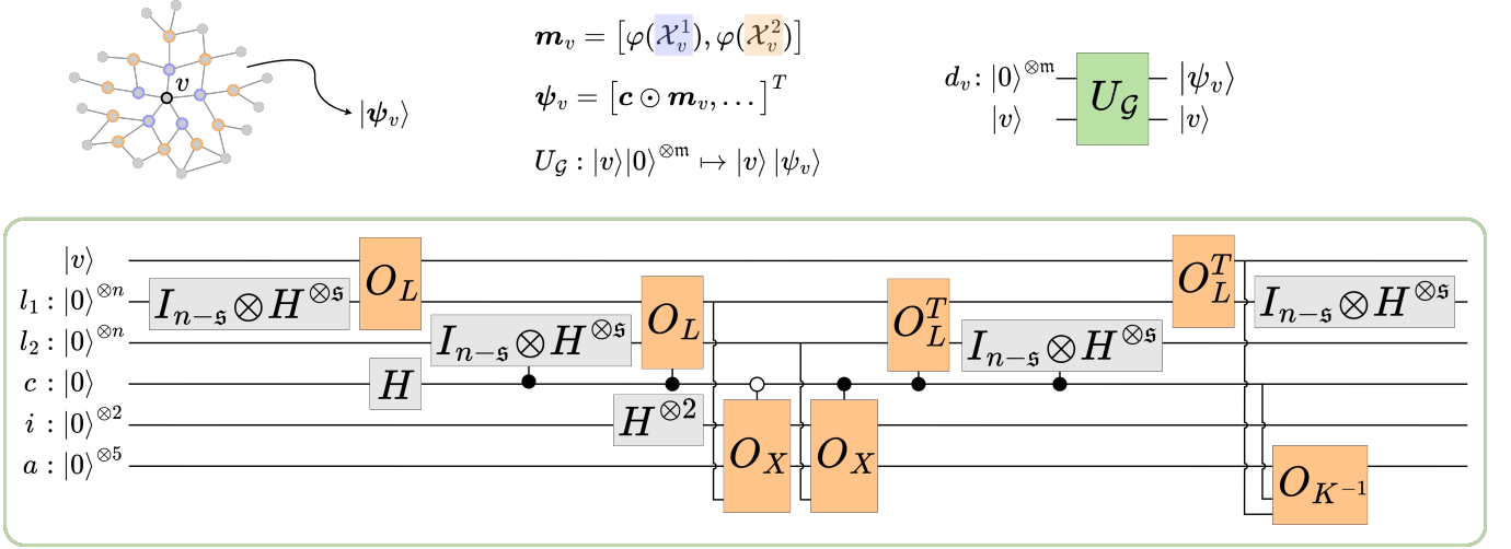
FIG. 2. Quantum Multi-order Moment Embedding (QMME) circuit schematic. The unitary operator U_{\mathcal{G}} : |v\rangle|0\rangle^{\otimes m} \mapsto |v\rangle|\boldsymbol{\psi}_v\rangle performs amplitude encoding of low-order statistical moments computed from the mutation scores of node v 's immediate and second-hop neighbors. Here, |v\rangle encodes the node index v \in V , and |0\rangle^{\otimes m} is the data register initialized to zero with m = \mathcal{O}(n) . The resulting quantum state |\boldsymbol{\psi}_v\rangle \in \mathbb{R}^{2^m} captures neighborhood statistics of the graph \mathcal{G} = (V, E, \mathbf{x}) for node v , based on the raw moment embedding function \varphi(\cdot) defined in eq. (9). The m -data register consists of the registers for neighbors l_1 and l_2 , a single qubit c indicating whether neighbors are immediate or second-hop, a two-qubit register i indexing the i -th moment, and a five-qubit ancilla register a . Input data includes real-world PPI networks with scalar node features such as mutation scores.
