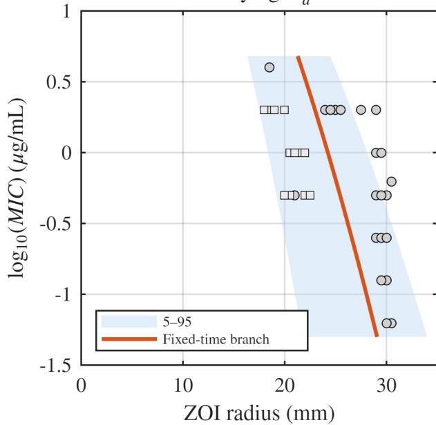
Varying D_a^*
