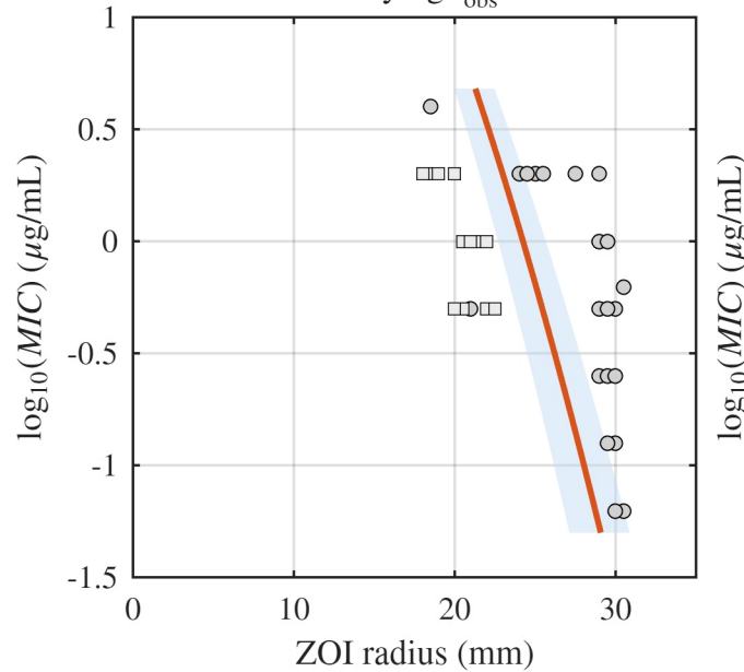
Varying t_{\text{obs}}^*
