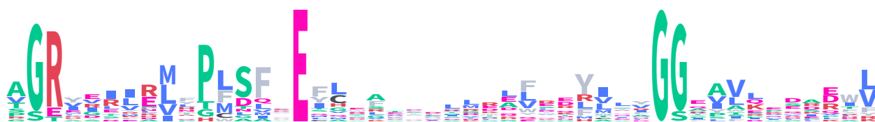
Sequence logo for positions 100–145 using the Dayhoff amino acid color palette.
